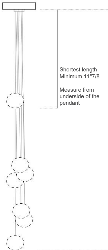
Cluster Column, Copper Suspension without Pendant Anchor Kit Configuration
